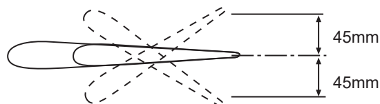
Rudder Control
