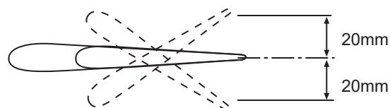
Aileron Control
