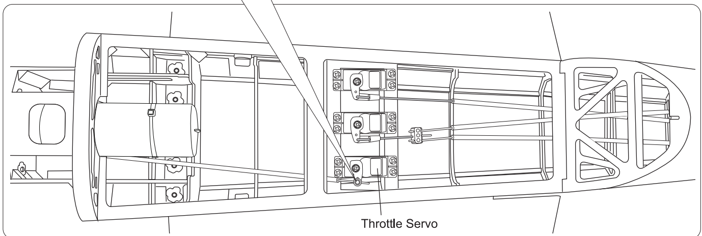
< Throttle Idling >
