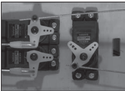
Low throttle
