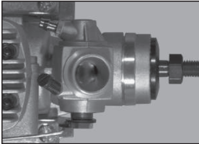
Low throttle
