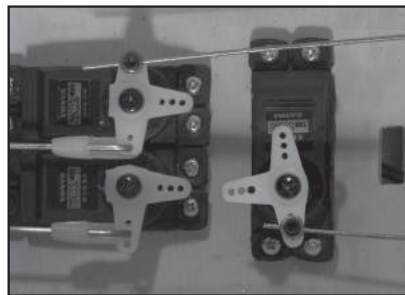
Mid throttle
