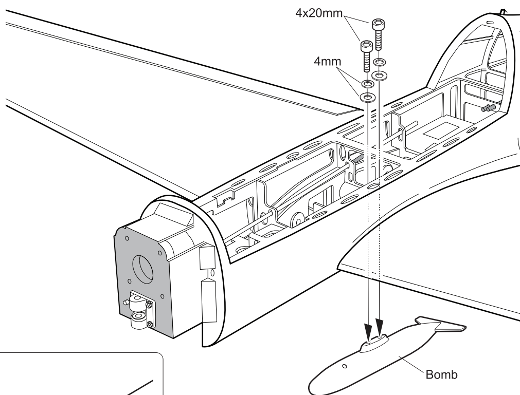
4 x 20mm Cap Screw
