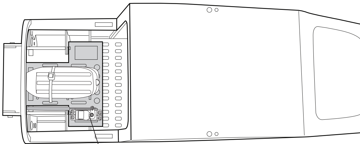
Throttle Servo
