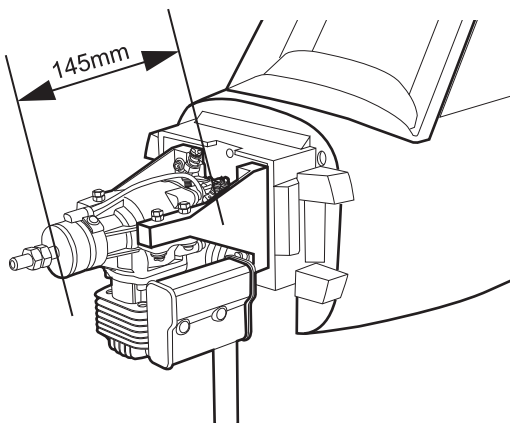
DLE 20cc with side exhaust
