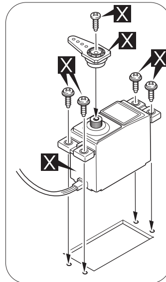
Rudder Servo
