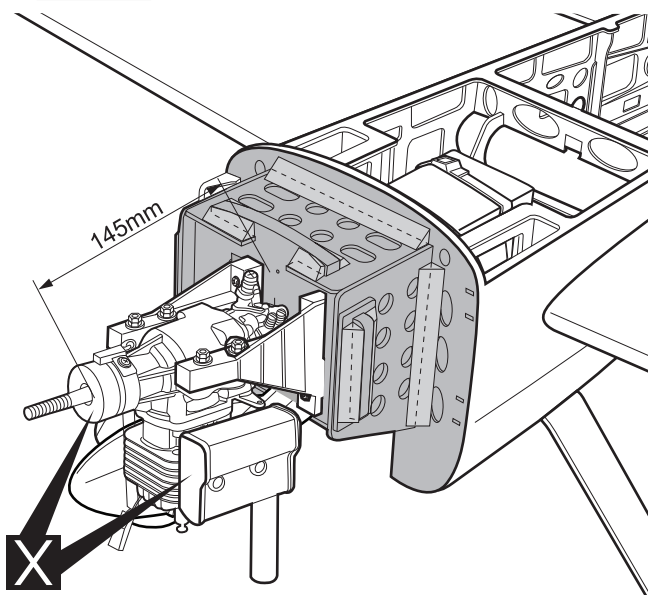
DLE-20
