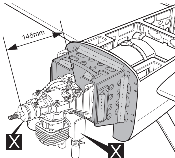
DLE-20RA
